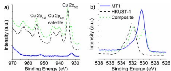
Figure 3. High-resolution XPS scans of MT1, HKUST-1 template, and the composite after crystallization. Normalized (a) copper and (b) oxygen spectra.
